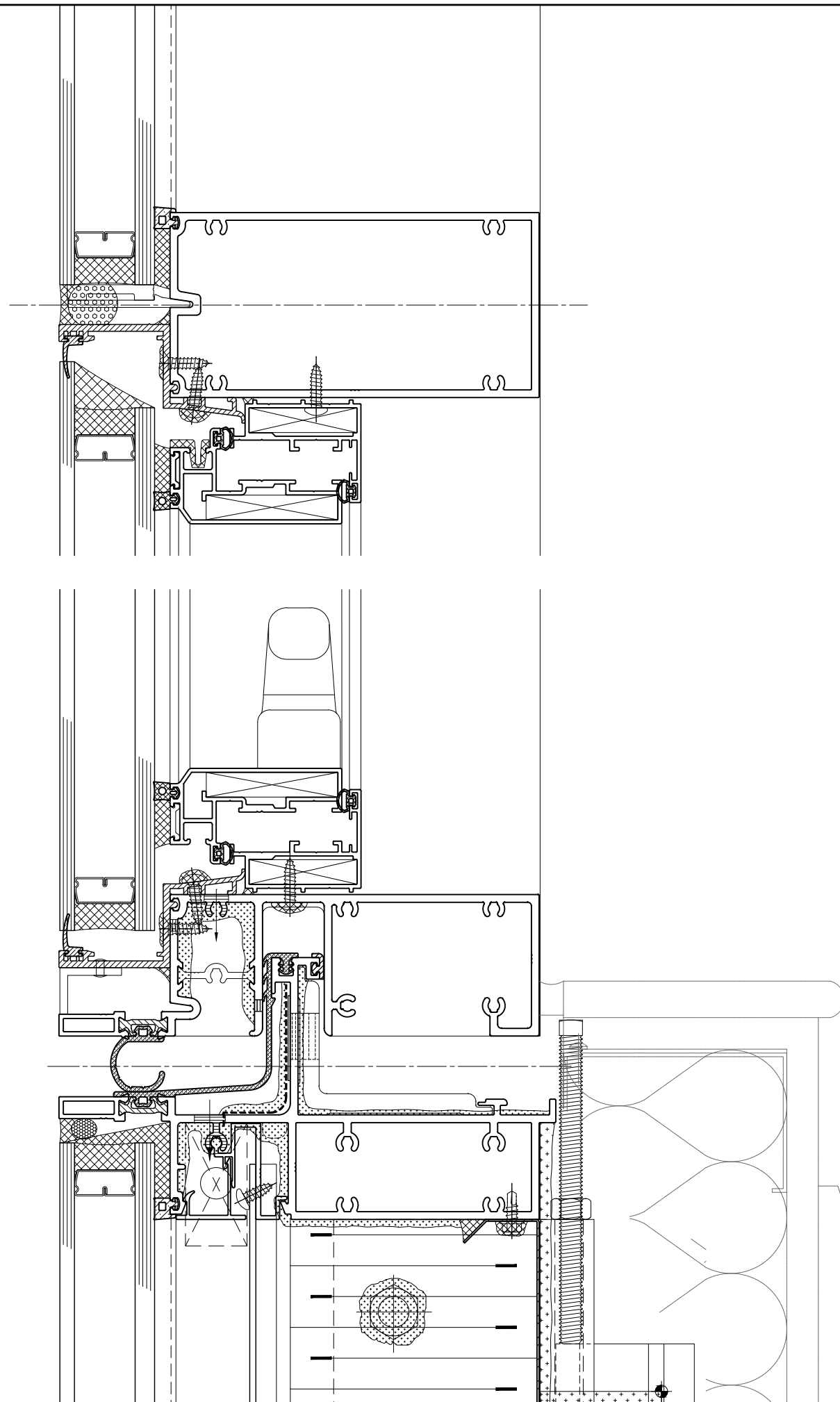
① TYPICAL SECTION DETAIL @ AWNING VENT
